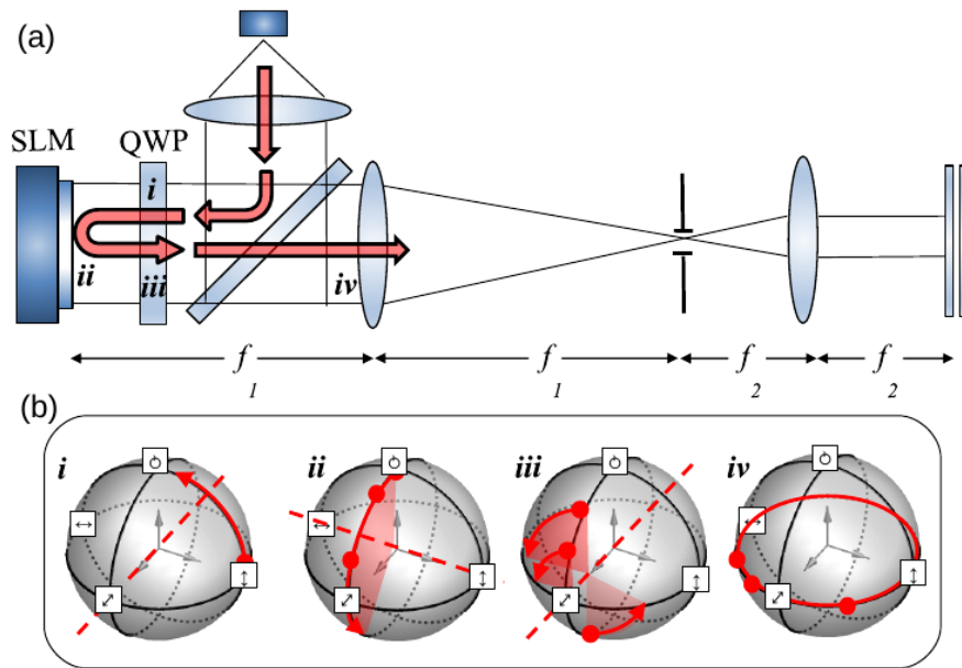
Fig. 2. (a) Optical train for polarization modulation, along with (b) the Poincaré sphere representation of its operation. (i) The initially s-polarized beam makes its first pass through the quarter-wave plate (QWP) with optic axis oriented at 45deg, and becomes circularly polarized. (ii) The beam is reflected from the LCoS spatial light modulator (SLM), each pixel of which acts as an independently variable waveplate. The accessible polarization states trace out an arc on the Poincaré sphere. (iii) A second pass through the QWP maps each of these polarization states back to a different linear polarization state. (iv) Crucially, as long as the retardance of the SLM pixels can be modulated through a full 2\pi of phase, all linear polarizations are accessible. Finally, the SLM plane is imaged onto the photoalignment cell, with a Fourier plane filter to reject higher diffracted orders.
